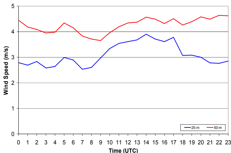
Diurnal Wind Speed Pattern
